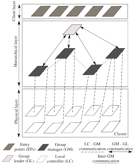
Fig. 1. System Architecture
