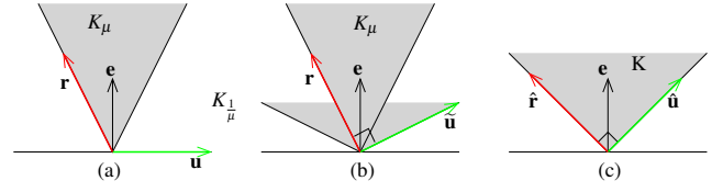
Figure 5: Successive changes of variables applied onto (a) the relative velocity \mathbf{u} and the contact force \mathbf{r} , in order to exhibit (b) the complementarity of \tilde{\mathbf{u}} and \mathbf{r} proposed by De Saxcé and Feng [1998], and (c) our new complementarity relationship between \hat{\mathbf{u}} and \hat{\mathbf{r}} on the self-dual cone K for a pure frictional contact ( \mu > 0 ).
