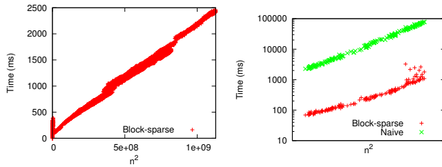
Figure 6: Computational time for assembling \mathbf{W} .
