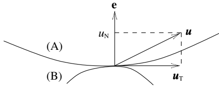
Figure 3: Local contact basis, with normal and tangent subspaces.
