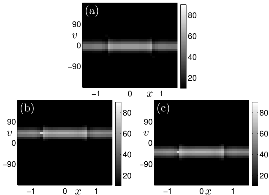
Figure 8: Three possible direction-selected solutions. Panels (a), (b) and (c) show, for \lambda = 14 , k = 0.3 , three possible direction-selected solutions corresponding to the unstable diagonal (D), stable vertical (V) and stable horizontal (H) percepts, respectively.
