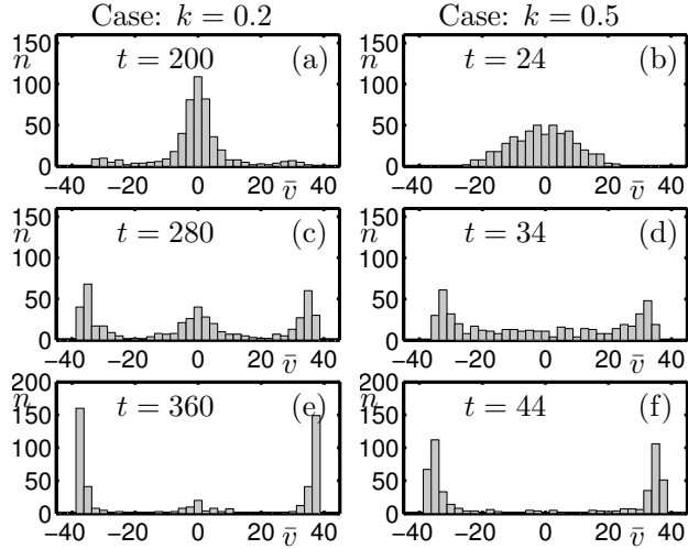
Figure 12: Histograms of the average direction \bar{v} taken at three different time snapshots for the two cases k = 0.2 and k = 0.5 for N = 500 trials.
