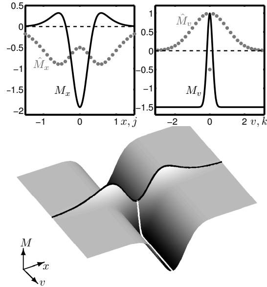
Figure 2: Profile of the connectivity function. (a) Form of the connectivity M_x in x -space and the corresponding Fourier transform \hat{M}_x . (b) Form of the connectivity M_v in v -space and the corresponding Fourier transform \hat{M}_v . (c) Full, coupled connectivity M . The functions M_x and M_v correspond to the 1D slices at v = 0 (black curve) and x = 0 (white curve), respectively.
