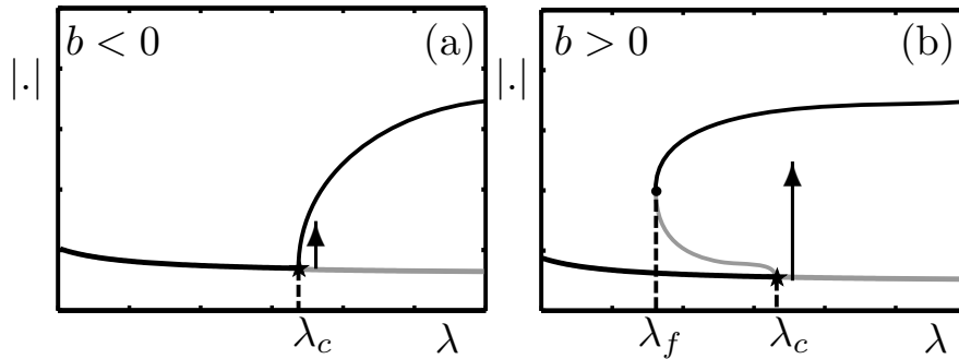
Figure 3: Sketch of bifurcation diagrams in \lambda for some norm ||\cdot|| of a (a) supercritical or (b) subcritical pitchfork. Lower solution branch corresponds to spatially homogeneous solutions, upper solution branch corresponds to direction-selected solutions; stable parts are black, unstable parts are grey. Pitchfork occurs at \lambda_c and in (b) there is a fold bifurcation on the direction-selected branch \lambda_f ; arrows indicate temporal dynamics when passing \lambda_c on the lower branch.
