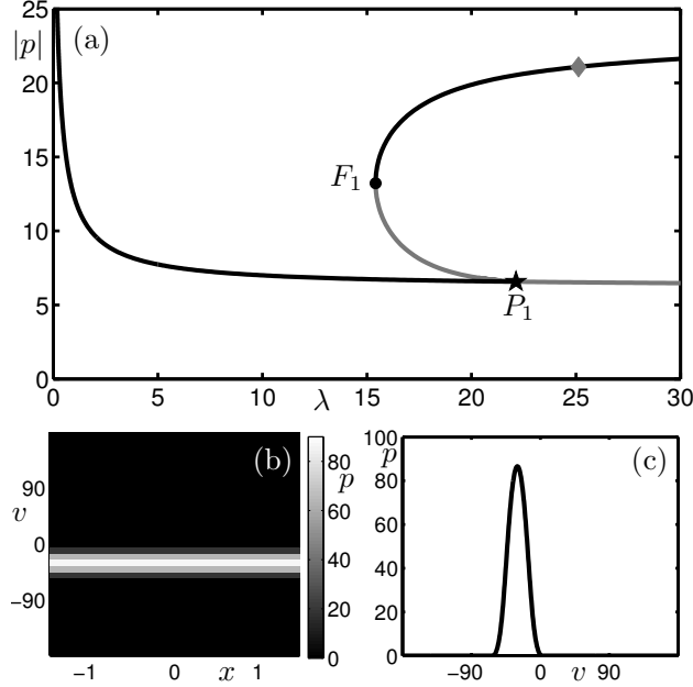
Figure 5: Model solutions in absence of stimulus. (a) A bifurcation diagram varying \lambda for k = 0 and the parameter values given in Table 1, where the solution norm is |p| ; branches of steady-state solutions are plotted with stable sections black and with unstable sections grey. The lower branch of solutions are spatially uniform in both x and v ; for increasing \lambda the branch loses stability in a subcritical pitchfork bifurcation at P_1 . The bifurcated branch represents direction-selected solutions (modulated in v but still uniform in x ); a change in stability occurs at the fold bifurcation F_1 . (b) Activity p plotted over the (x, v) -plane for the direction selected solution indicated by a diamond marker on the upper branch in panel (a). (c) Cross section in v at an arbitrary value of x from panel (b).
