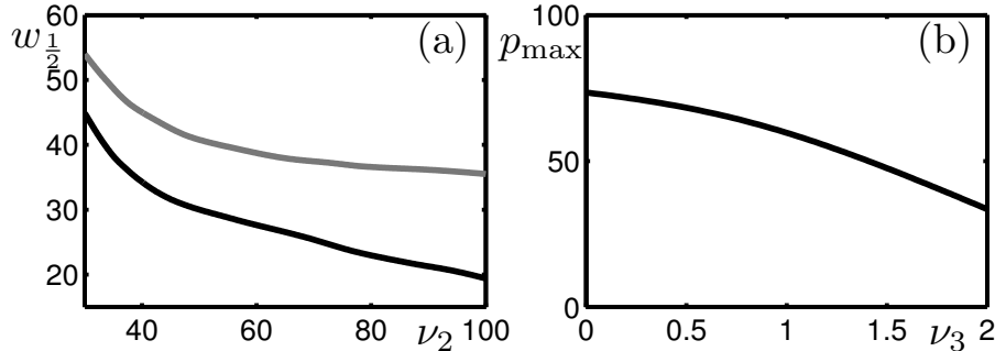
Figure 6: Tuning of parameters \nu_2 and \nu_3 . (a) Dependence of velocity tuning half-width w_{\frac{1}{2}} on \nu_2 at fold point F_1 ; black curve computed for \nu_3 = 0 , grey curve computed for \nu_3 = 1.5 . (b) Dependence of maximum activity level for direction-selected solutions p_{\max} on \nu_3 computed for \nu_2 = 66 .
