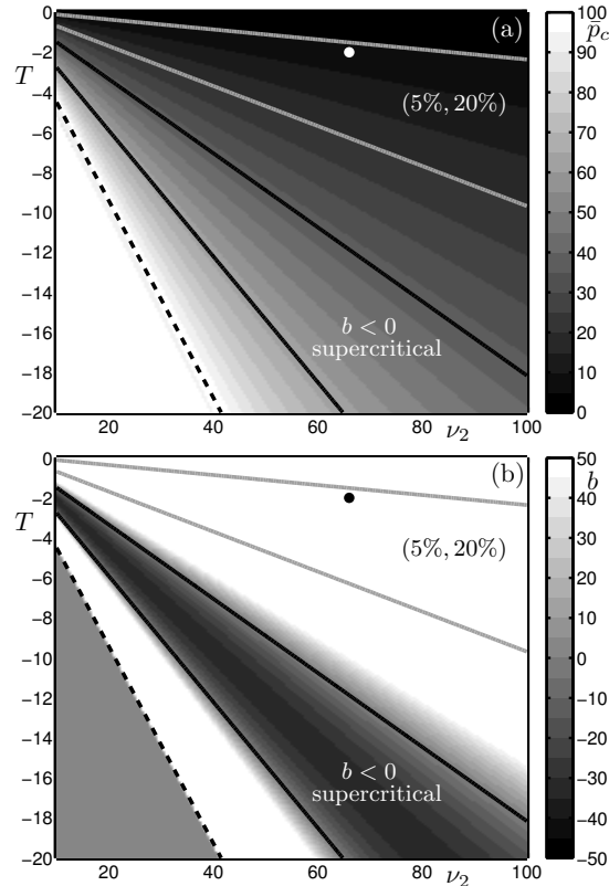
Figure 4: Tuning the parameters T and \nu_2 . (a) Grey scale map of activity level \bar{p}_c at bifurcation point \lambda_c ; plotted in both panels are the contours 5% and 20% (grey) along with the contour 99% (dashed black). (b) Grey scale map of the normal form coefficient b as given by equation Eq. (23); plotted in both panels are the contours b = 0 (black); positive values correspond to a subcritical bifurcation and negative values to a supercritical bifurcation. For |T| large (white region in bottom left of (a), grey region in bottom left of (b)) the activity level is saturated at \bar{p}_c = 100\% and b \approx 0 because the Taylor coefficients S_* \approx 0 .
