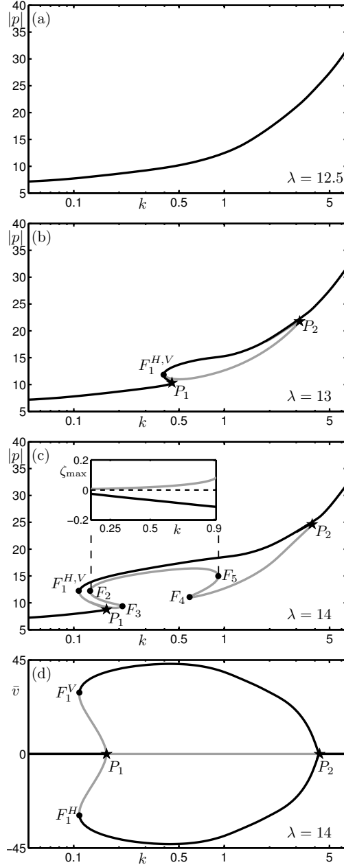
Figure 7: Branches of steady-state solutions are plotted for varying bifurcation parameter k (shown on a logarithmic scale) as computed for different values of \lambda ; stable sections of solution branches are black and unstable sections are grey. Changes in stability occur at fold bifurcations (black points) and pitchfork bifurcations (black stars). In panels (a), (b) and (c) solutions are plotted in terms of the L_2 -norm of the solution vector |p| for \lambda = \{12.5, 13, 14\} , respectively. The inset in panel (c) shows the largest eigenvalue \zeta_{\max} along the two upper solution branches from the main panel over the range of k as indicated by vertical dashed lines. Panel (d) shows the same solution branches as in panel (c), but in terms of the average direction \bar{v} .
