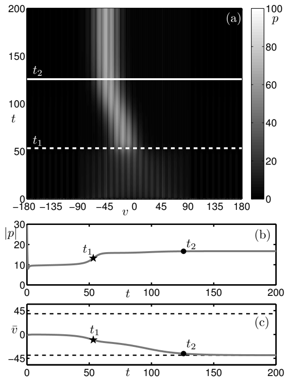
Figure 10: Example of temporal dynamics for (\lambda, k) = (14, 0.3) initialised from random initial conditions. (a) Grey scale map showing the evolution activity levels p(x, v, t) with time on the vertical axis. The state vector p is indexed locally by position in physical space x and globally by position in direction space v and it is, therefore, convenient to show v -position on the horizontal axis. At the time-point labelled t_1 (horizontal white dashed line, star in panels (b) and (c)) there is a transition to the diagonal direction-selected solution. At the time-point labelled t_2 (horizontal white line, point in panels (b) and (c)) there is a transition to the final steady-state, direction-selected solution. (b) Time-evolution of |p| ; the time-mark t_1 is the point of steepest increase for |p| . (c) Time evolution of the average direction \bar{v} with horizontal dashed black lines indicating the two possible final steady-state solutions. The time-mark t_2 is taken as the first point where the \bar{v} is within 3^\circ of the final selected direction.
