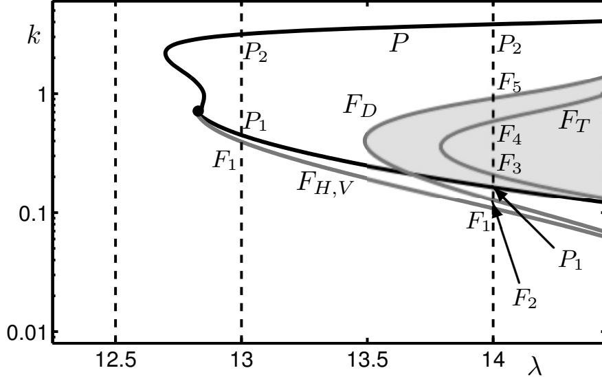
Figure 9: A two-parameter bifurcation diagram is shown in the (\lambda, k) -plane where the locus of pitchfork bifurcation P is a black curve and the loci of fold bifurcations F_{H,V} , F_D and F_T are a grey curves. The point where the coinciding fold curves F_{H,V} terminate at an intersection with the pitchfork curve P is indicated by black point. One-parameter slices indicated by vertical dashed lines correspond to the bifurcation diagrams for fixed \lambda and varying k shown in Fig. 7; the labels along these slices correspond with the bifurcation points in Fig. 7.
