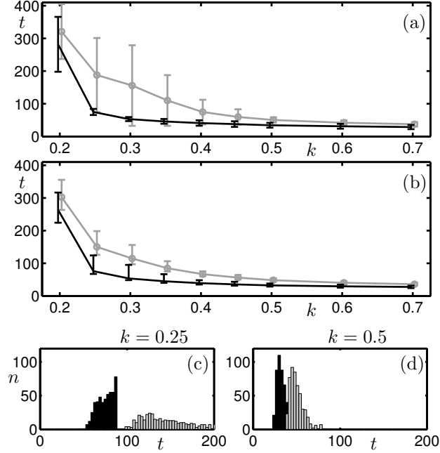
Figure 11: Variability and skewness of the time-marks t_1 and t_2 dependent on the parameter k . At each k -value the data from N = 500 simulations with random initial conditions is shown. (a) Mean value of t_1 is plotted in black and of t_2 in grey over a range of values of k with error bars showing the standard deviation. (b) Similarly, the median is plotted with error bars showing the first and third quartile of the distributions. (c), (d) Example histograms of t_1 in black and t_2 in grey for k = 0.25 and k = 0.5 , respectively.
