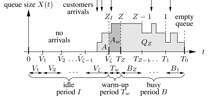
Figure 1: Sample trajectory of the queue size during a regeneration cycle.
