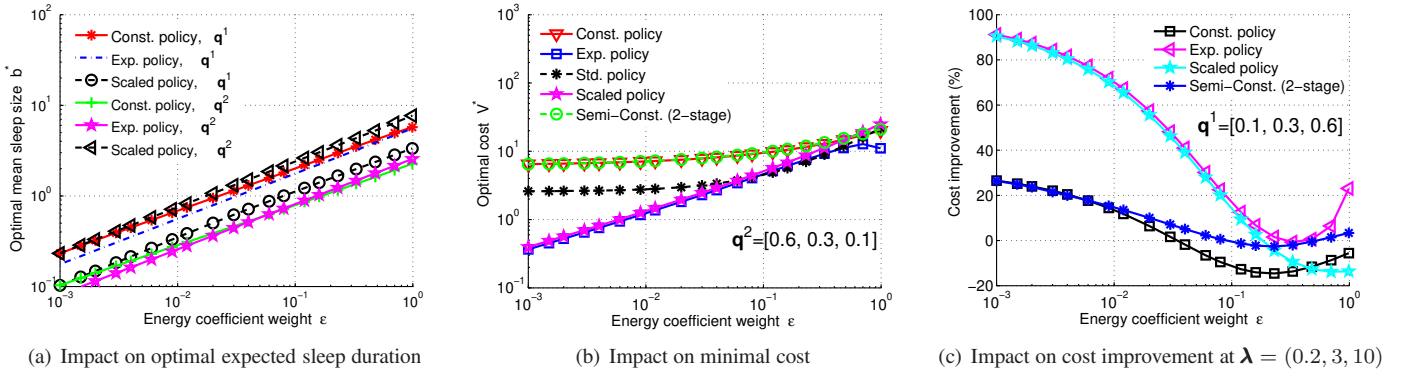
Figure 4: Hyper-exponential \tau : Impact of \epsilon for various sleep policies.
