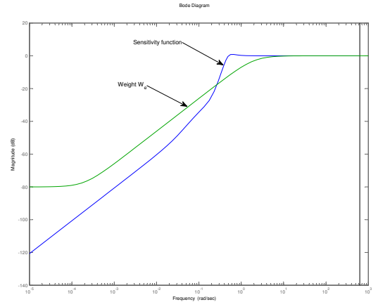
Fig. 4. Sensitivity functions of the pitch control
