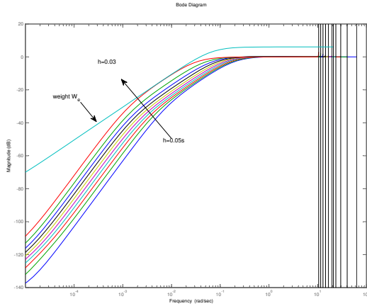
Fig. 7. S sensitivity function
