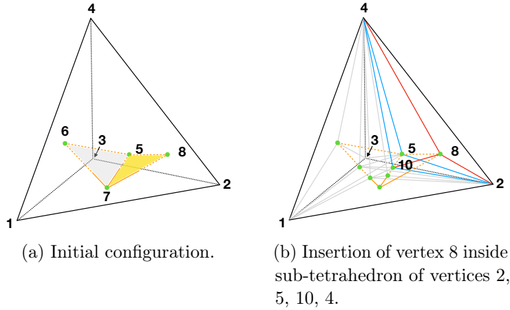
Figure 2.12: Step I.3.1 for solid triangle 8, 5, 7 : insertion of solid vertices 8, 5, 7 inside tetrahedron \{1, 2, 3, 4\} , which is already been intersected from the solid triangle \{5, 6, 7\} . Vertices 5 and 7 are already been inserted, vertex 8 is internal to the sub-tetrahedron \{2, 5, 10, 4\} , hence, is divided in 4 sub-tetrahedra.
