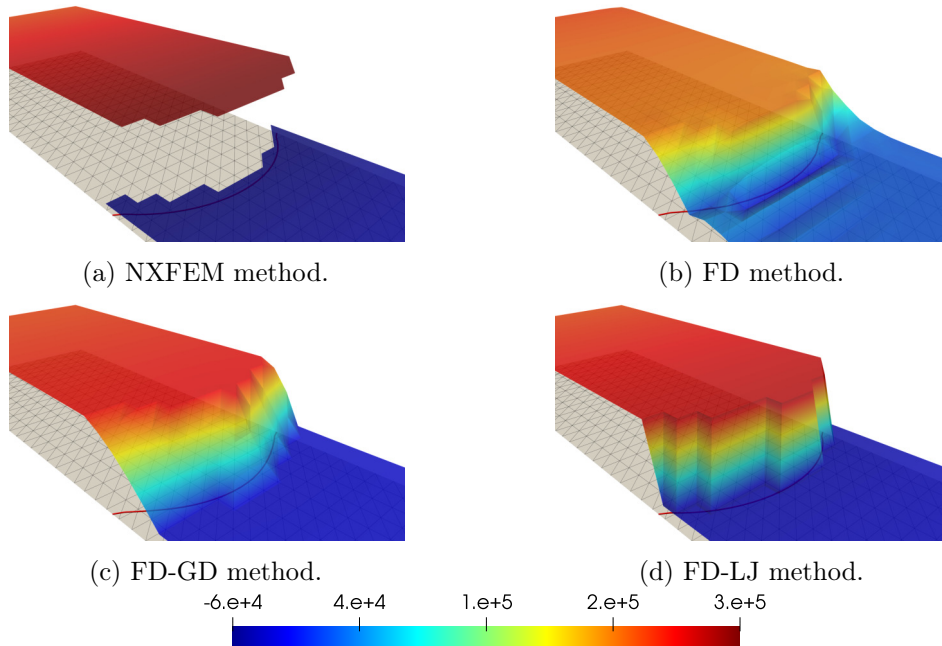
Figure 4.12: Snapshots of the fluid pressure at t = 0.125 for the M1 refinement level.
