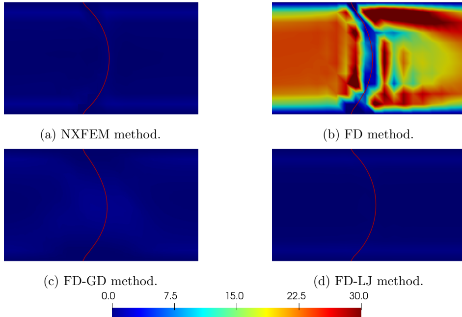
Figure 4.9: Snapshots of the fluid velocity magnitude at t = 0.125 for the M1 refinement level.
