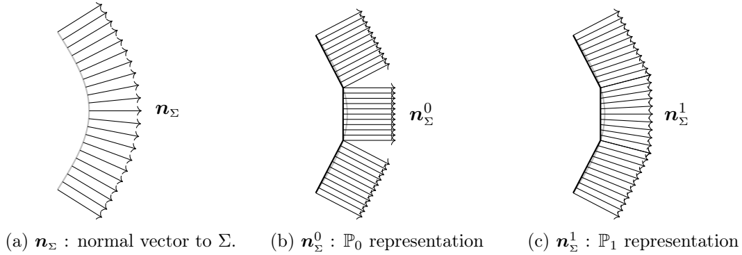
Figure 3.6: Geometric approximation of the normal vectors to the interface \Sigma . In gray the interface \Sigma and in black the mesh \mathcal{T}_{\mathcal{H}}^{\Sigma} .
