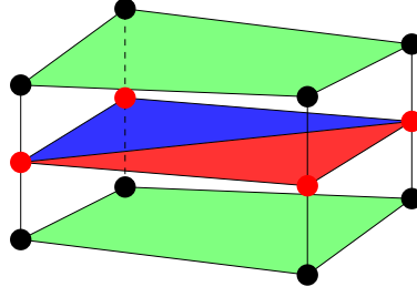
Figure 4.3: Example of the elements composing \mathcal{T}_\mathcal{H}^\Sigma (red and blue triangles), and \mathcal{T}_\mathcal{H}^{\Omega^s} (green hexahedra).
