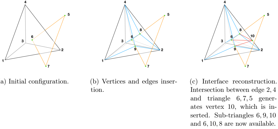
Figure 2.15: Reconstruction of structure sub-triangles after further solid triangle and fluid edges intersection.
