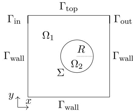
Figure 4.26: Lid-driven cavity geometric configuration.
