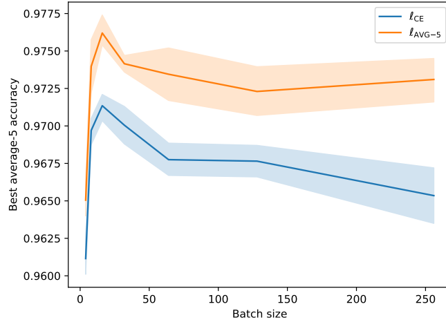
Figure 5.6: CIFAR-100 best validation average-5 accuracy as a function of batch size for a DenseNet 40-40 trained with \ell_{AVG}^{5,\alpha} or \ell_{CE} . For a fair comparison we maintain the ratio of learning rate to batch size constant. The 95% confidence interval is represented.
