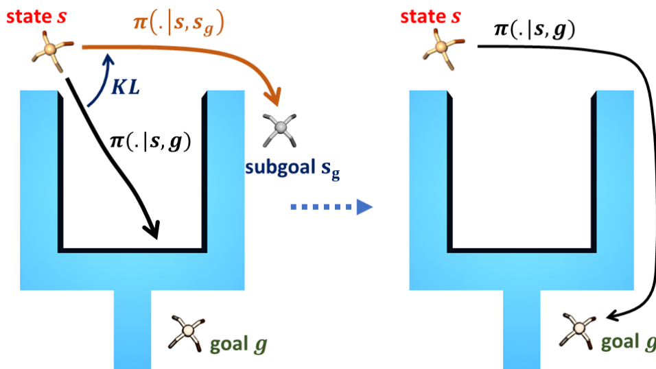
Figure 3.1 – Illustration of the KL-regularized policy learning using imagined subgoals. (Left): The policy fails to reach a distant goal, yet it can reach a closer subgoal. Our approach automatically generates imagined subgoals for a task and uses such subgoals to direct the policy search during training. (Right): At test time, the resulting flat policy can reach arbitrarily distant goals without relying on subgoals.
