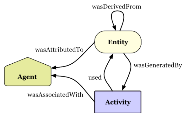
Figure 16: Overview of the W3C PROV model
