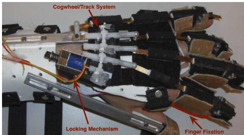
Figure 3.2: Prototype of a hybrid orthosis for assisting the power grasp from [118].
