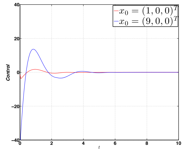
(c) Control inputs.
