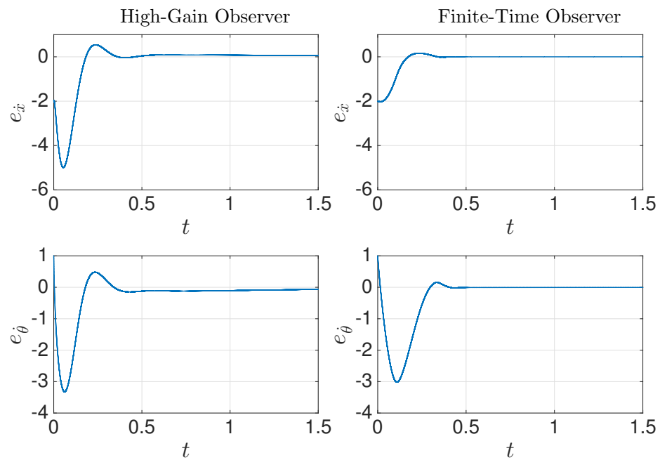
Figure 2.2: Simulation plots of e_{\dot{x}} and e_{\dot{\theta}} for the HG and finite-time observers applied to the nonlinear plant with IC x(0) = (0, -2, \frac{\pi}{4}, 1) and K_p = 10 .
