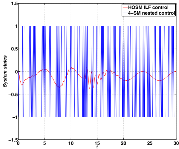
(c) Comparison of control inputs.
