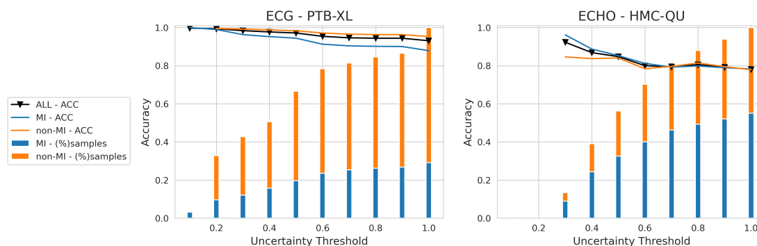
Fig. 6.3.: The change of prediction accuracy with respect to uncertainty threshold on PTB-XL ECG dataset and HMC-QU ECHO dataset (2CH/4CH mixed). Bar plots represent the percentage of samples kept under varying uncertainty thresholds.
