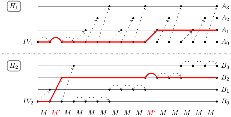
Figure 2.8: Using the interchange structure to reach output (A_1, B_2) .
