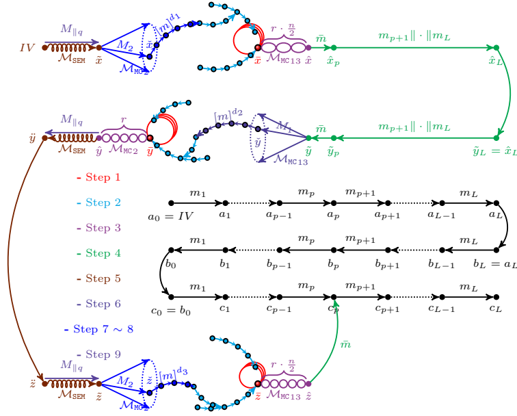
Fig. 10: Second-preimage attacks on 3-pass Zipper
