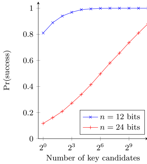
Fig. 3. Results for lists size of 3 \cdot 2^{2n/3}
