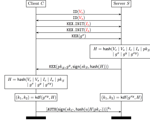
Fig. 8. SSH-2: Key exchange and user authentication.
