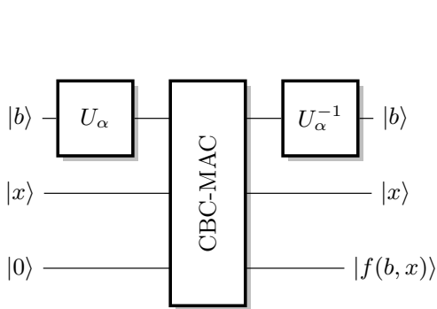
Fig. 10. Simon's function for CBC-MAC.
