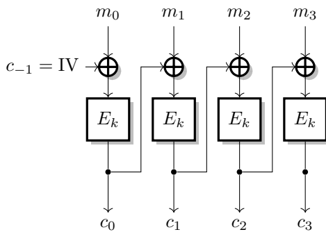
Figure 5.1: CBC mode.
