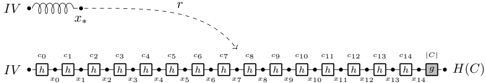
Figure 2.4: Second-preimage attack.
