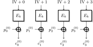
Figure 3: CTR mode
