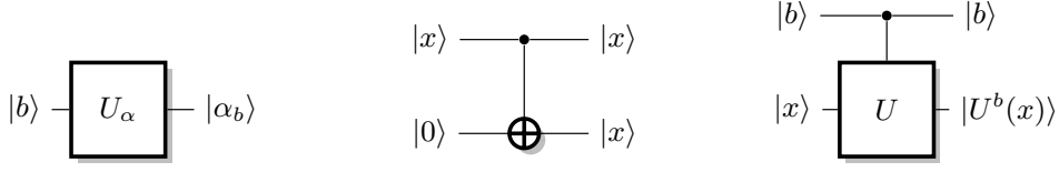
2.1. One-to-one mapping.
