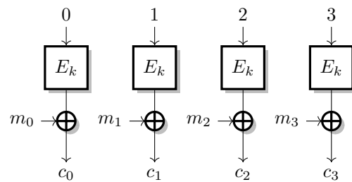
Figure 5.2: CTR mode.
