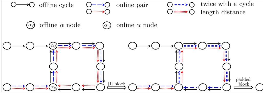
Fig. 2. Distinguishing-H attack
