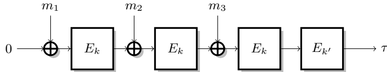
Fig. 9. Encrypt-last-block CBC-MAC.
