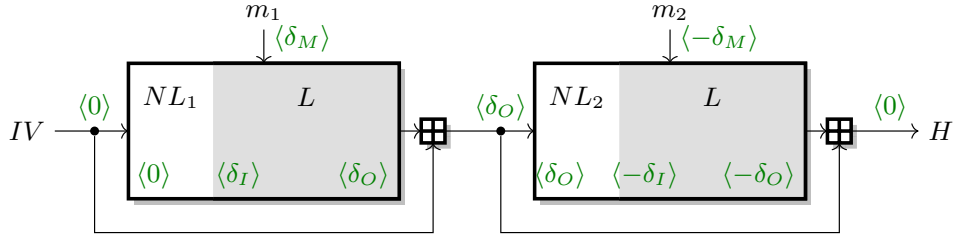
Fig. 1. 2-block collision attack using a linear trail \delta_I \overset{\delta_M}{\rightsquigarrow} \delta_O and two non-linear trails 0 \rightsquigarrow \delta_I and \delta_O \rightsquigarrow -\delta_I . Green values between bracket represent differences in the state.
