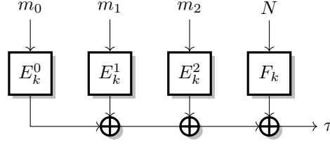
Figure 7.5: \Theta\text{CB3} used as a MAC.
