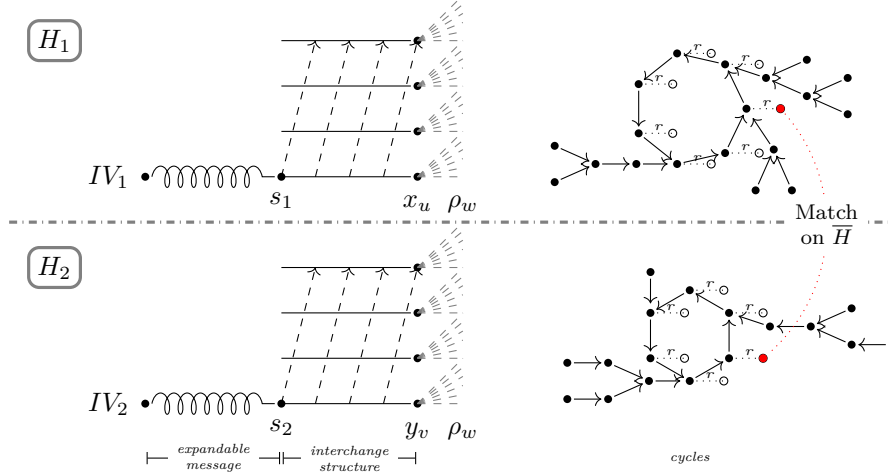
Figure 2.10: Improved preimage attack on the XOR combiner based on cycles.
