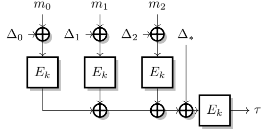
Figure 7.3: PMAC' variant.
