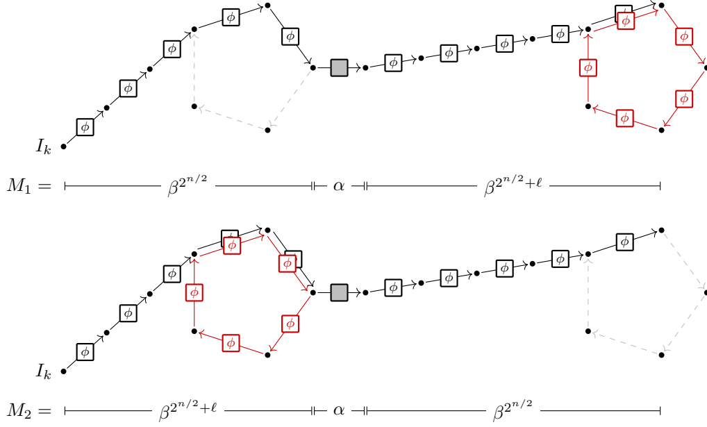
Figure 4.2: Cycle-based collision.
