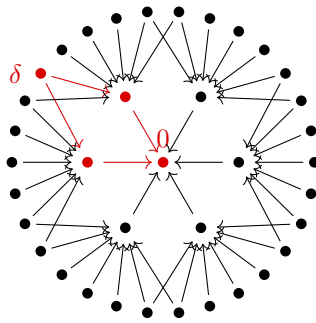
Figure 3.7: With clustering.
