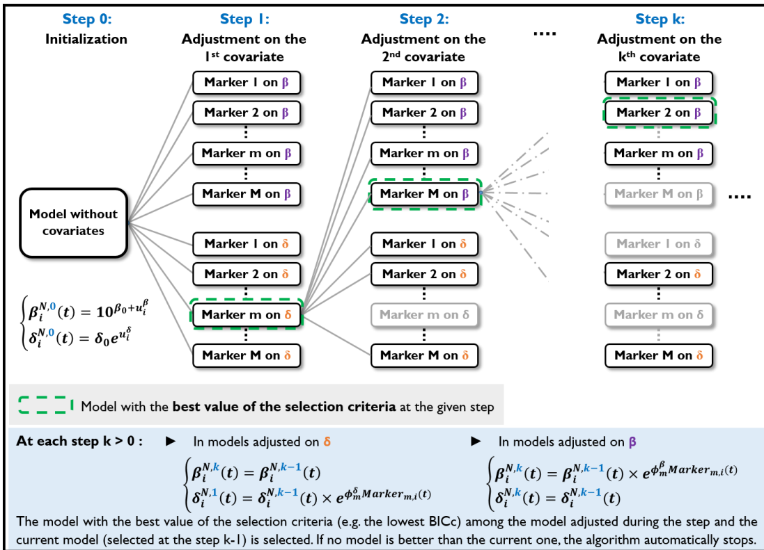
1195 Figure 4 - figure supplement 2. Flow chart of the algorithm for automatic selection of covariate.
