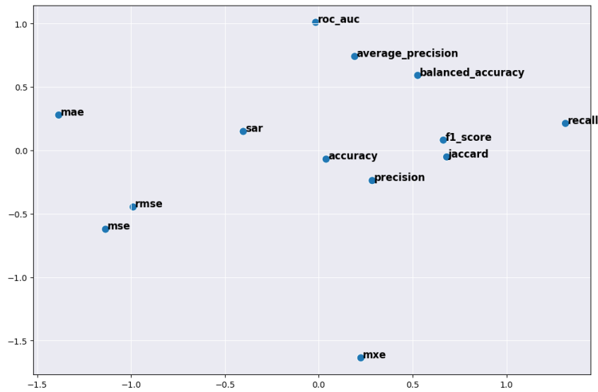
Figure 4.2 – Multidimensional scale (MDS) plot illustrating the degree of correlation between scoring metrics in a 2D space. The metrics are compared by computing Euclidean distance between the rankings they produced. This experiment was performed on the classification tasks and models from AutoDL Challenge (presented in Section 8.1).
