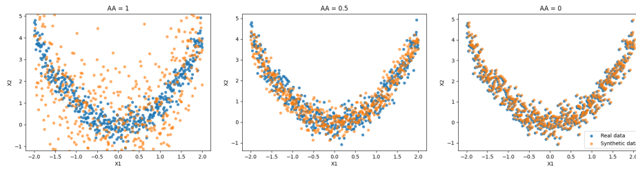
Figure 4.3 – Adversarial Accuracy (AA) is the performance of an nearest neighbor classifier that distinguishes between real data vs synthetic data . The ideal value is AA = 0.5 (represented by the plot in the middle). This is a bi-variate ( X_1 and X_2 ) illustrative example.
