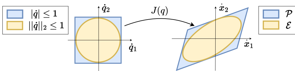
FIGURE 7.1: An example manipulability polytope and ellipsoid geometry for a planar m = 2 robot with n = 2 . The difference between the Joint Space (JS) limits for ellipsoid described with \|\dot{\mathbf{q}}\|_2 \leq 1 (orange) and the range limits -\mathbf{1} \leq \dot{\mathbf{q}} \leq \mathbf{1} (blue) is shown on the right. The difference in obtained achievable task-space velocity \dot{\mathbf{x}} polytope \mathcal{P} (blue) and ellipsoid \mathcal{E} (orange) is shown on the right plot. The plots show that both in joint and task-space the ellipsoid metric is an underestimation of the true robot’s capacity.
