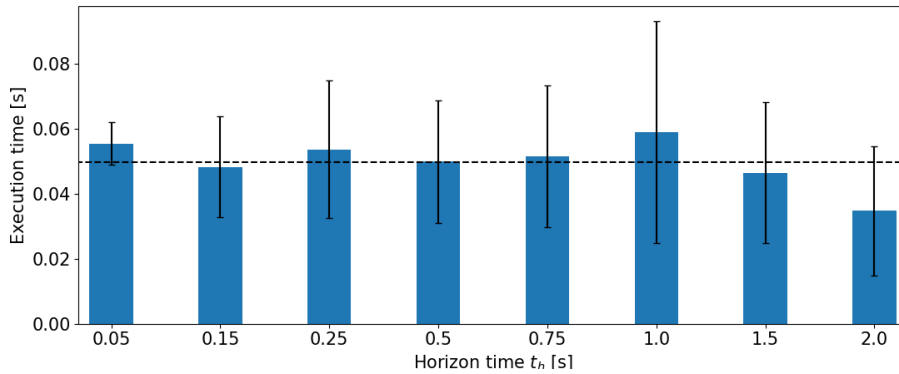
FIGURE 5.12: Execution time of the polytope \mathcal{P}_x enumeration using ICHM algorithm. Average and standard deviation calculated over 1000 executions for each of the 8 horizon lengths.
