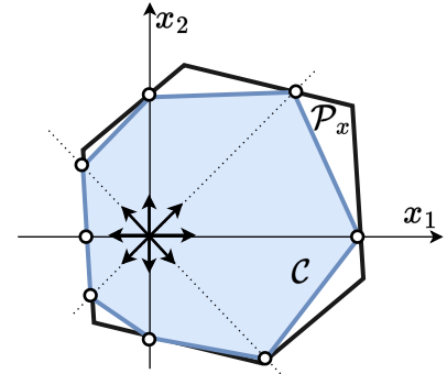
FIGURE 3.13: An example of the approximation \mathcal{C} of the 2D ( m = 2 ) polytope \mathcal{P}_x using a RSM algorithm. The input space is sampled with 8 rays.
