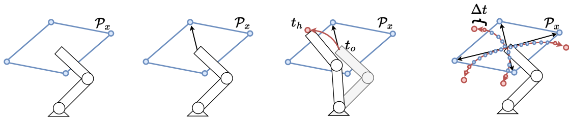
FIGURE 5.9: Images show the steps (left to right) of the nonlinear simulation procedure on a simplified 2 link planar robot. First the polytope \mathcal{P}_x of the end-effector is determined. For each \mathbf{x}_{v_i} vertex of the \mathcal{P}_x , the joint torque \boldsymbol{\tau}_{v_i} , generating this vertex, is applied to the robot simulation (figures in the middle). All the robot's end-effector positions \mathbf{x}_k in all the simulation time steps \Delta t are saved for further analysis.
