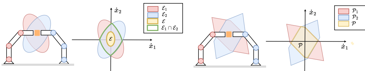
FIGURE 1.3: Comparison of using ellipsoids (left) and polytopes (right) for collaborative physical ability calculation. Using polytopes, the common velocity capacity of the two robots is calculated as the intersection of their polytopes \mathcal{P} = \mathcal{P}_1 \cap \mathcal{P}_2 . In ellipsoid case the intersection of the ellipsoids (green) is no longer an ellipsoid and it is hard to characterise, while the collaborative ellipsoid \mathcal{E} (orange) introduced by Chiacchio et al. [10] is a large underestimation of the true joint capacity.
