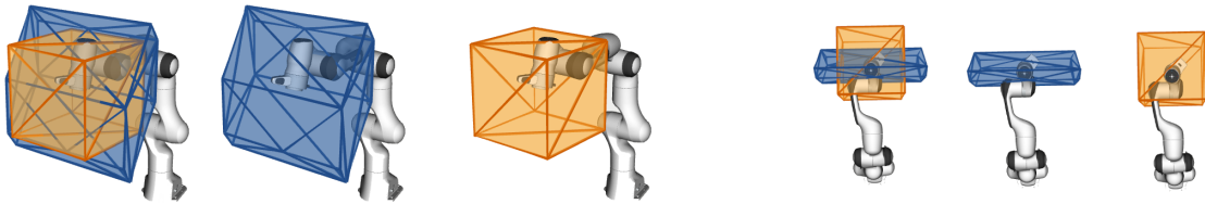
FIGURE 5.11: Comparison of the end-effector reachable space approximation using the convex polytope \mathcal{P}_x (blue) and the cube \mathcal{C}_x (orange) for the Panda robot with the horizon time t_h=200\text{ms} .
