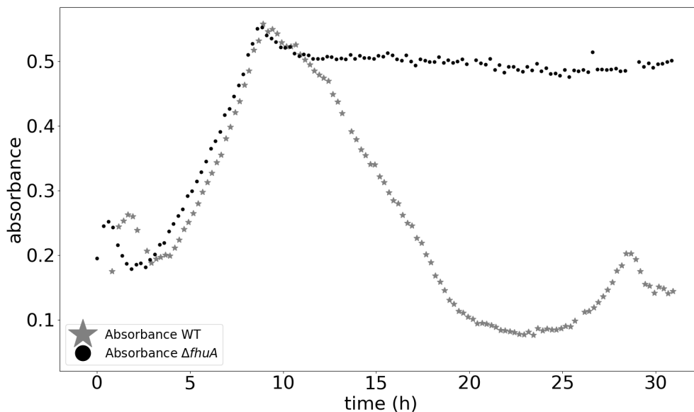
Figure 23: Absorbance dynamics for the WT and the FhuA knock-out in chemostat. The FhuA knock-out is in steady-state from 11 to 30 hours, whereas the WT culture collapses immediately after having reached steady-state.
