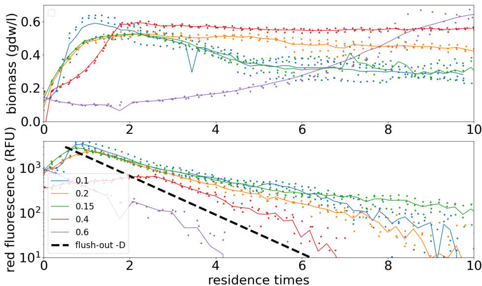
Figure 35: Dynamics of total biomass (upper panel) and red fluorescence (lower panel) at increasing dilution rates. To compare experiments properly, time is rescaled in residence time units. The lines represent the mean of three technical replicates, whose values are indicated by the dots. The black dashed line indicates the expected flush-out if the cells were simply flushed out by the dilution rate. The slope of this flush-out is independent of the dilution rate because time is rescaled in residence time units.
