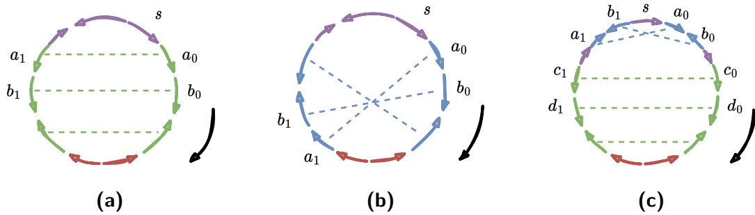
■ Figure 32 – Chloroplast repeat scaffolding.
