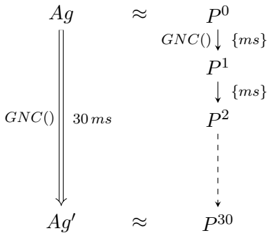
(a) GNC semantics simulation diagram
