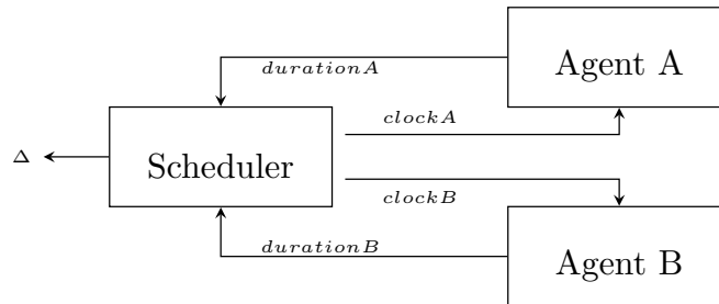
Figure 8.2 – Temporal optimization architecture
