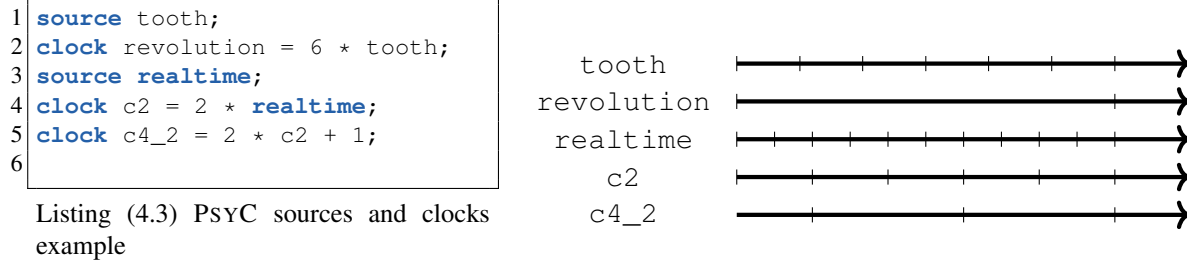
Figure 4.3 – The left part shows the PSYC syntax the source and clock example, and the right part shows a possible chronogram of their execution
