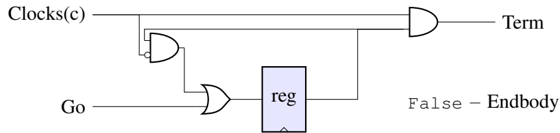
Figure 7.3 – Circuit modeling of the advance 1 with c statement of PSYC
