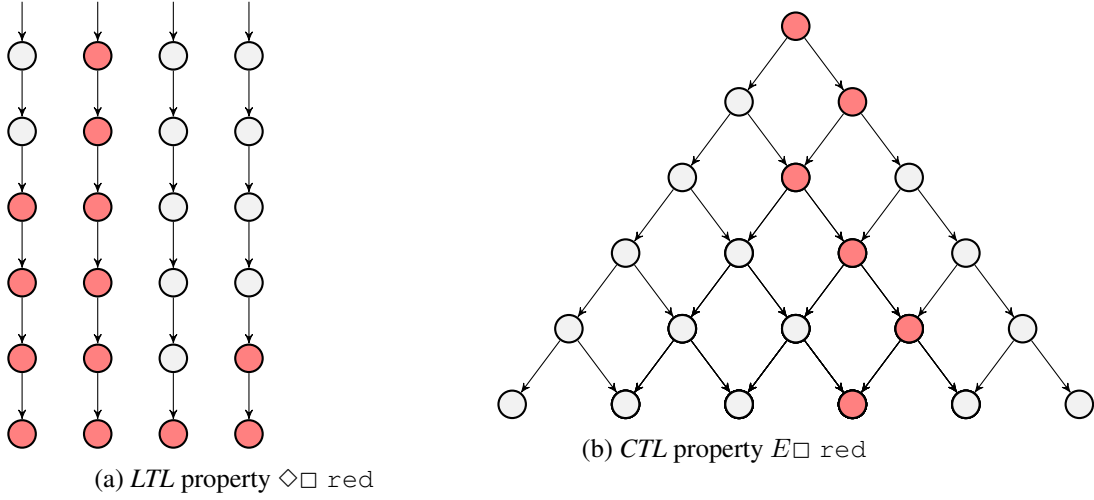
Figure 3.6 – LTL and CTL property examples
