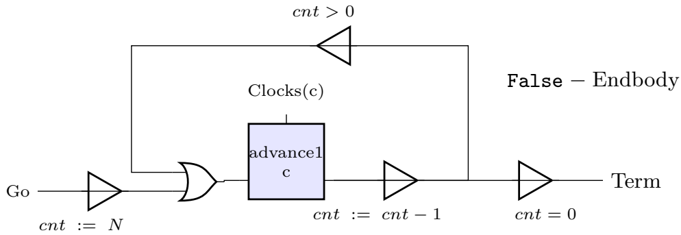
Figure 7.4 – Circuit of the advance n with c statement of PSYC
