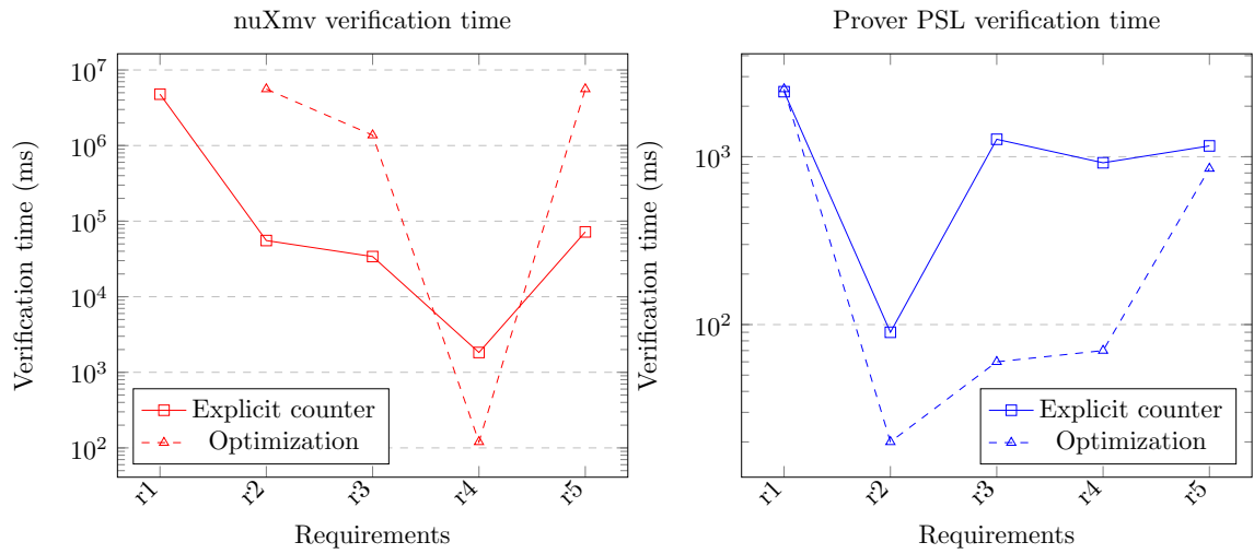
Figure 8.4 – The leftmost plot and the rightmost plot show the verification time for respectively nuXmv and Prover PSL. Absent values denote timeout (2h).
