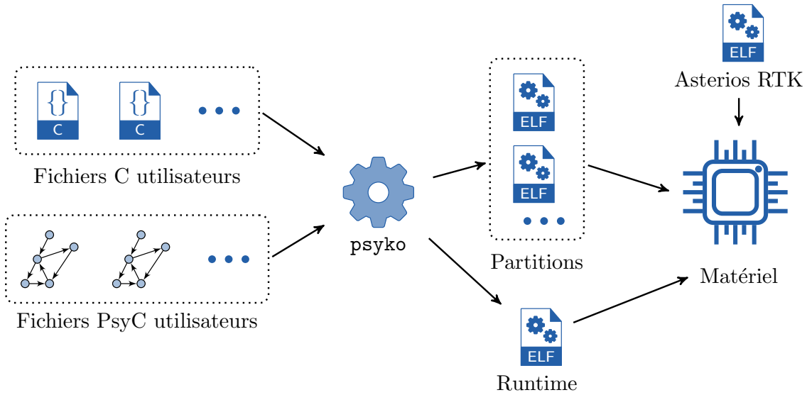
Figure 4.1 – PSYC toolchain overview
