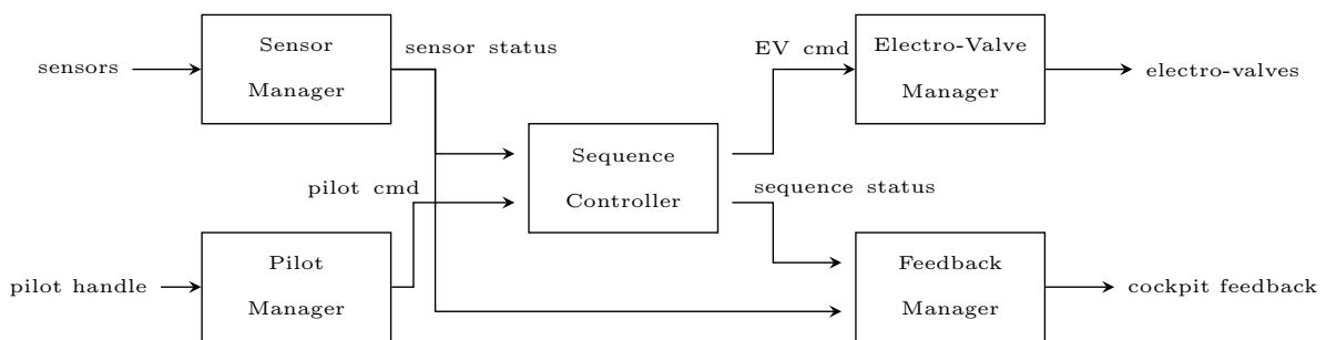
Figure 8.3 – The Landing Gear System (LGS) functional architecture
