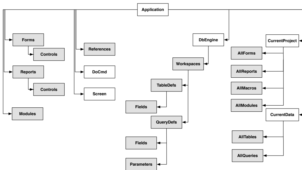
Figure 5.2: Access COM Object model. In white, those elements we can use directly. In grey, those elements depend on other elements and specific interactions.
