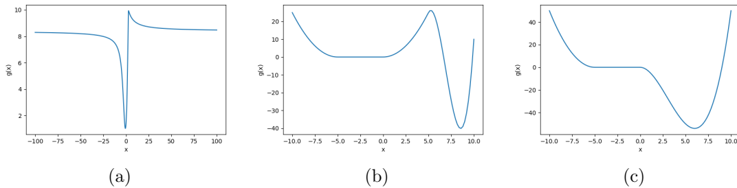
Figure 4.1: Examples of functions with spurious objects.
