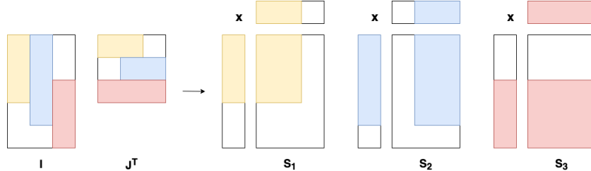
Figure 5.1: Illustration of the idea of support of rank-one contribution. Colored rectangles indicate the support constraints (I, J) and the support constraints \mathcal{S}_k on each component matrix \mathbf{X}[:,k]\mathbf{Y}[:,k]^\top .
