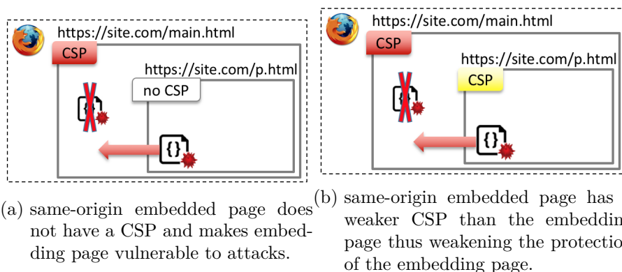
Figure 2.1: Fundamental problem of Content Security Policies (CSP) in embedded pages. If either embedded (resp. embedding, not shown here) page has no CSP or a weaker CSP than embedding (resp. embedded) page, the overall protection of the Web application is set by the weakest CSP (or no CSP).
