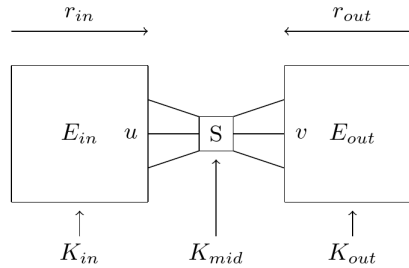
Figure 1.4: Sieve-in-the-middle framework
