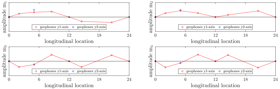
Figure 7.6 – First four modeshapes of the testing bridge.
