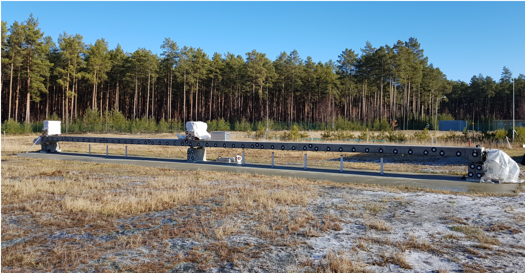
Figure 7.1 – Testing bridge.
