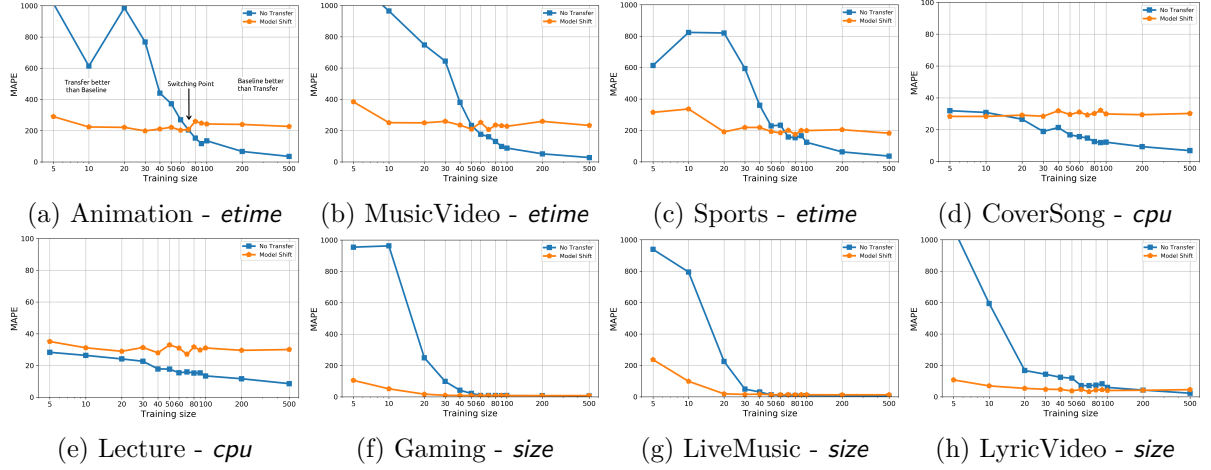
Figure 7.5 – Mean Average Percentage Error (y-axis, lower is better) when transferring x264 to x265 performance depending on the training size (x-axis, log scale), for eight input videos and three performance properties
