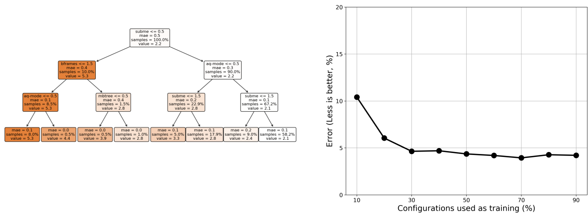
(c) Predicting performance out of configurations
