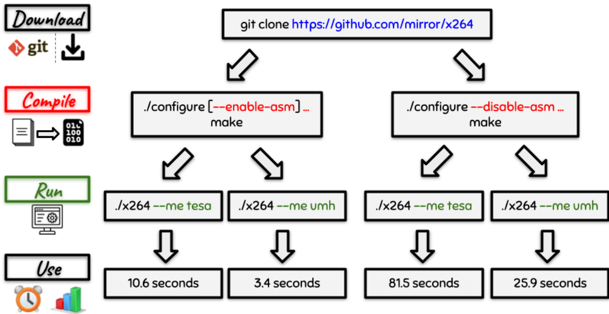
Figure 5.1 – Cross-layer variability of x264
