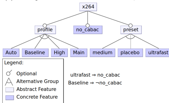
(c) Constraints of the --no-cabac option
