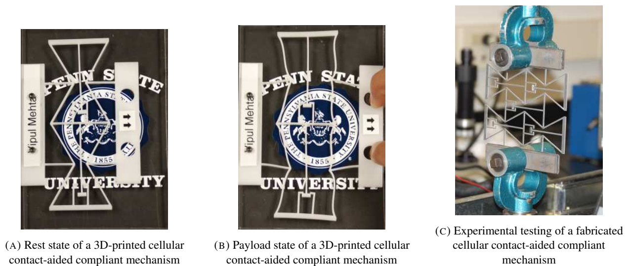
FIGURE 1.9: Contact-aided compliant mechanisms (Mehta, 2010)
