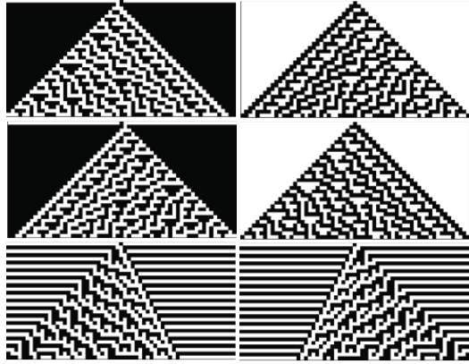
(a) 6 highest scoring automata. Only the first 30 timesteps are shown for readability.
