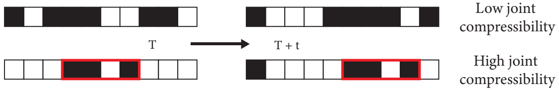
Figure 4.2 – Joint compression method illustration. If a structure persists through time, this will decrease the joint compressed length compared to the sum of compressed lengths. A persistent structure is circled in red.
