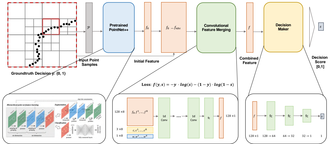
Figure 2.22 – Network structure of the neural occupancy prediction component.
