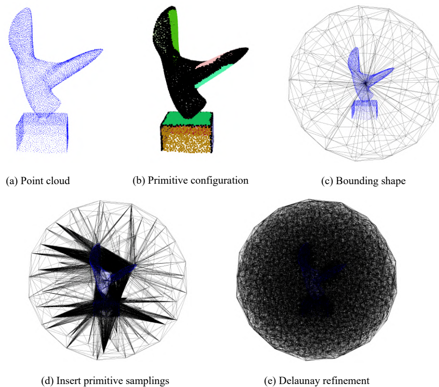
Figure 3.5 – Primitive-aware domain initialization for an input 3D point cloud.
