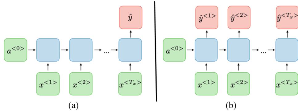
Figure 6.5 RNN architectures used popularly in satellite time series image based crop classification: (a) Many to one, and (b) Many to many RNN architectures [250].
