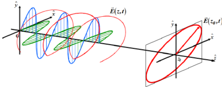
Figure 1.5 Illustration of the propagation of an electromagnetic plane wave. The electric field vector has horizontal (green) and vertical (blue) components, which combine to yield the net electric field vector (red) [27].
