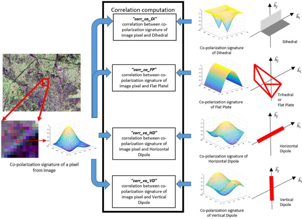
Figure 3.6 Figure illustrates the computation of polarization signature correlation features (PSCFs) between observed (image pixel) and standard targets PSs.
