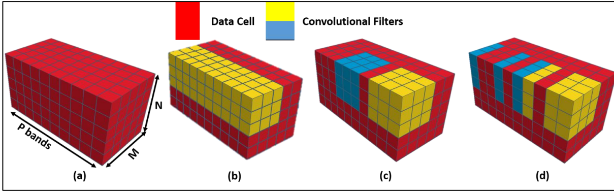
Figure 5.5: Different convolution strategies: (a) Data cuboid with M by N pixels and P bands, (b) Convolution with 3 \times 3 \times P convolutional filter where 3 \times 3 represents the spatial extent and P represents the total number of bands in the data. Each filter convolves with all the bands. This strategy is employed in 2D CNNs, (c) Convolution with 3 \times 3 \times 3 convolutional filters where 3 \times 3 represents to the spatial extent and 3 represents number of adjacent bands to be convolved simultaneously. One filter can convolve with three adjacent bands only. This strategy is employed in 3D-CNNs [96], and (d) Convolution with 3 \times 3 \times 3 convolutional filters where 3 \times 3 represents the spatial extent and 3 represents the number of arbitrarily selected bands to be involved. This strategy is employed in the proposed Perm-LSS-CNN framework.
