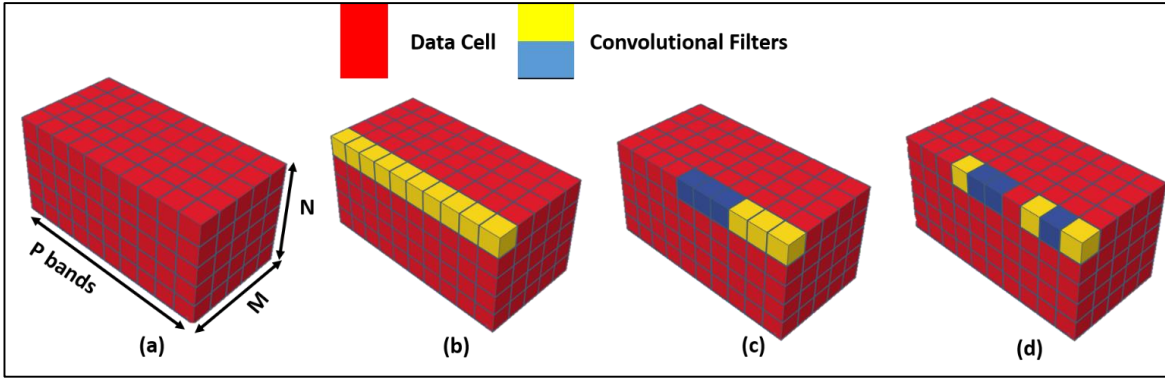
Figure 5.4 Different convolution strategies: (a) Data cuboid with M by N pixels and P bands, (b) Convolution with 1 \times 1 \times P convolutional filter where 1 \times 1 represents to the spatial extent and P represents total number of bands in the data. Each filter convolves with all the bands as all times. This strategy is employed in 1D-CNNs during per pixel classification of satellite images. (c) Convolution with 1 \times 1 \times 3 convolutional filters where 1 \times 1 represents the spatial extent and 3 represents the number of adjacent bands to be convolved simultaneously. One filter can convolve with three adjacent bands only. This strategy is also employed in 1D-CNNs. (d) Convolution with 1 \times 1 \times 3 convolutional filters where 1 \times 1 represents to the spatial extent and 3 represents number of arbitrarily selected bands to be involved. This strategy is employed in the proposed Perm-LS-CNN framework.
