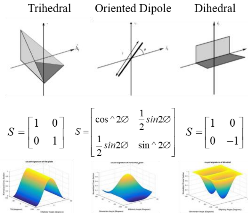
Figure 3.5 Geometrical structures, scattering matrices, and co-polarization signatures of different standard targets.
