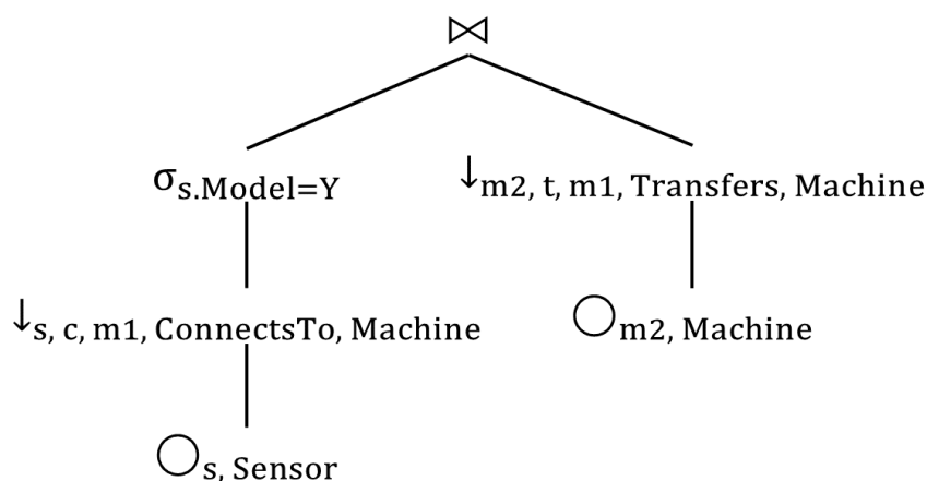
Figure 2.2 – Possible evaluation plan of the query Q
