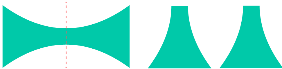
Figure 27: Print with overhanging features cut to be printed without supports.
