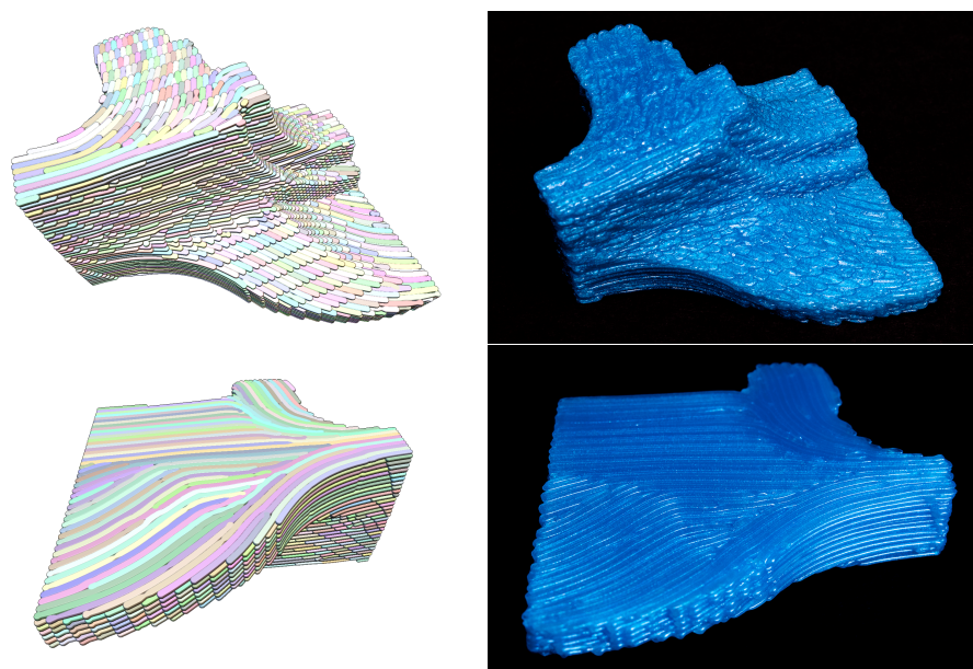
Figure 67: A mechanical part. A view from below is provided in the second row to highlight the input direction field.
