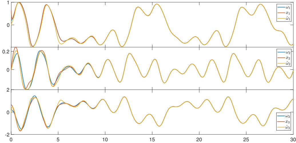
FIGURE 3.7: Simulation results for example 4 (2a,2b). Initial conditions: \omega(0) = (0.2 \ 0 \ 0.2)^\top , x(0) = (0.65 \ 0 \ \frac{1}{2})^\top , \hat{\omega}(0) = (0 \ 0 \ 0)^\top .
