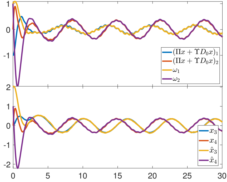
FIGURE 3.8: Example 5. Reduced-order observer for a mass-spring system.
