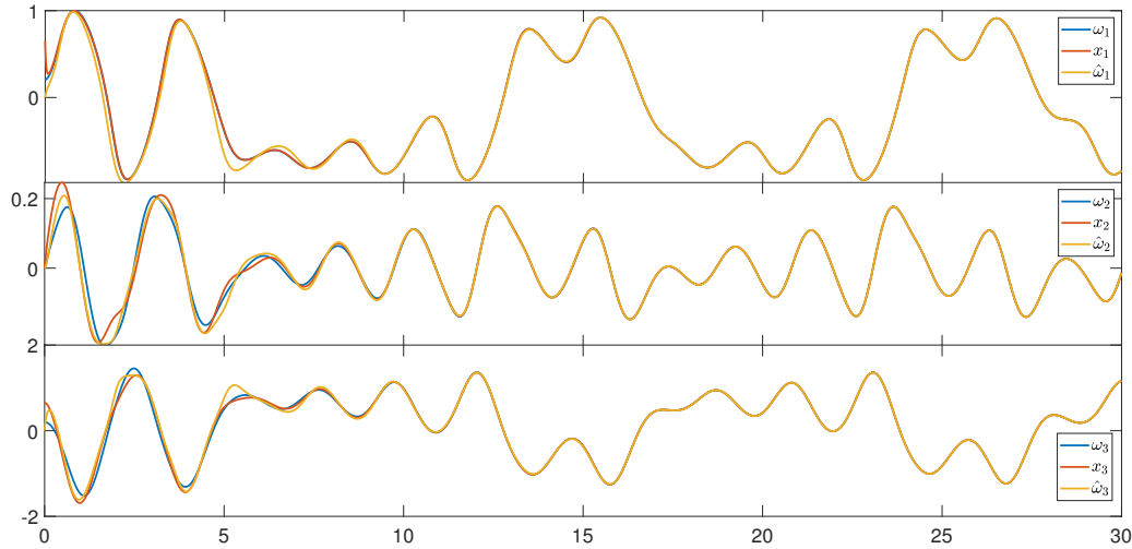
FIGURE 3.8: Simulation results for example 4 (2a,2b). Initial conditions: \omega(0) = (0.2 \ 0 \ 0.2)^\top , x(0) = (0.65 \ 0 \ \frac{1}{2})^\top , \hat{\omega}(0) = (0 \ 0 \ 0)^\top .
