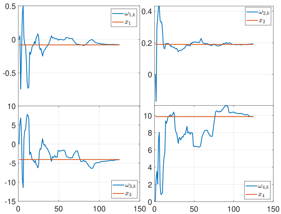
FIGURE 3.11: Parameter's convergence for Example 7
