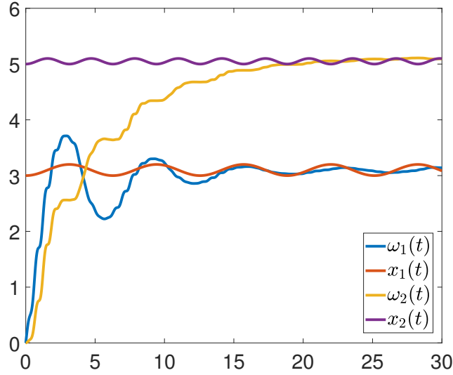
FIGURE 3.10: Example 2: nonlinear regression for a system given in a form (3.50).
