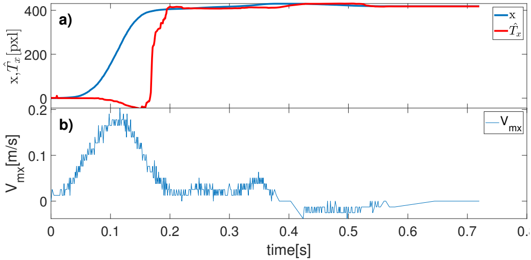
FIGURE 2.6: Correction phase model estimation: a) t [s] vs x and \hat{T}_x [pxl]; b) t [s] vs V_{mx} [m/s]
