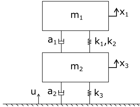
FIGURE 4.3: Schematics for Example 9
