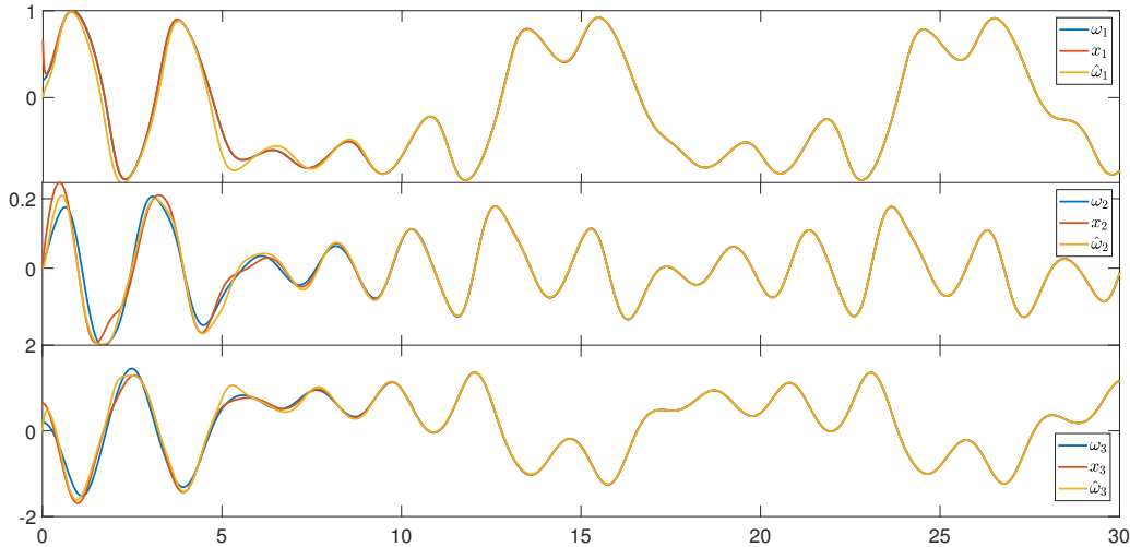
FIGURE 3.8: Simulation results for example 4 (2a,2b). Initial conditions: \omega(0) = (0.2 \ 0 \ 0.2)^\top , x(0) = (0.65 \ 0 \ \frac{1}{2})^\top , \hat{\omega}(0) = (0 \ 0 \ 0)^\top .
