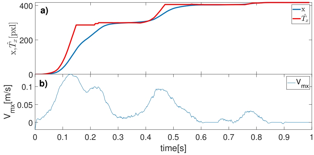
FIGURE 2.8: Switched model estimation for one trial: a) t [s] vs x and \hat{T}_x [pxl]; b) t [s] vs V_{mx} [m/s]
