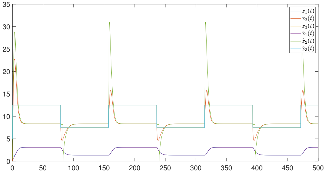
FIGURE 3.6: Observer for example 9. Initial conditions: \hat{x}(0) = (0.5 \ 0.5 \ 5)^T , x(0) = (1 \ 0 \ 5)^T , m = (0 \ 4 \ 0)^T
