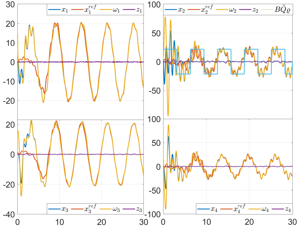
FIGURE 3.7: Observer for example 3. Initial conditions: z(0) = (0 \ 0 \ 0 \ 0)^T , \omega(0) = (15 \ 15 \ 15 \ 15)^T , x(0) = x^{ref}(0) = (0 \ 0 \ 1 \ 0)
