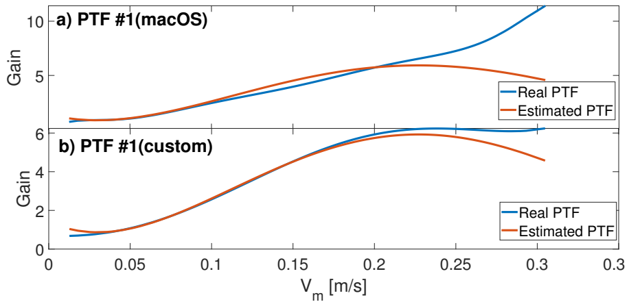
FIGURE 2.13: Gains comparison: V_m [m/s] vs gain
