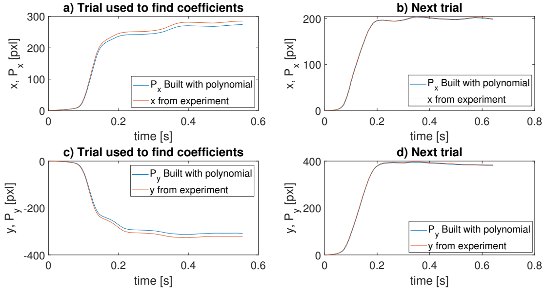
FIGURE 2.12: Transfer functions: x, y [pxl] vs time
