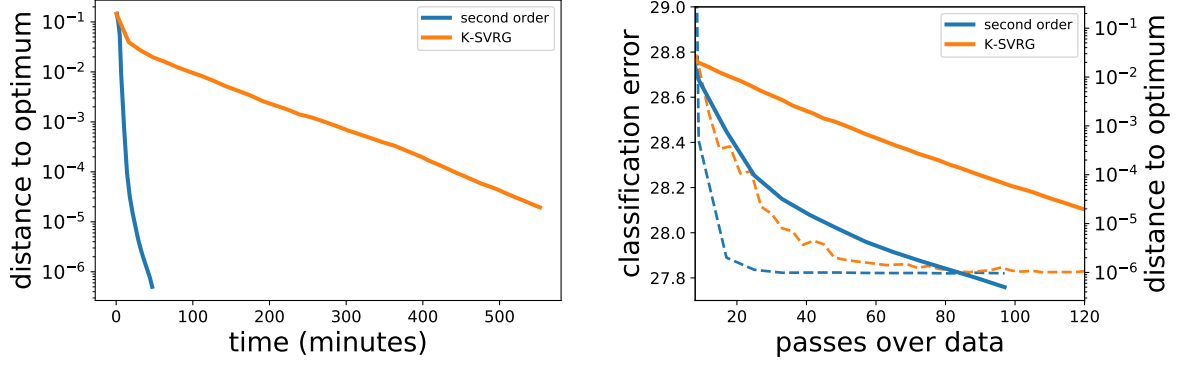
Figure 5.4: (Left) Distance to optimum as a function of time and (Right) distance to optimum and classification error as a function of the number of passes on the data when performing our second order scheme and K-SVRG to minimize the train loss on Higgs, with 1.0 \times 10^4 Nyström points and \lambda = 10^{-9} .
