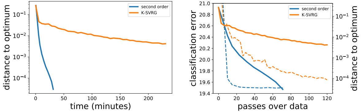
Figure 5.5: (Left) Distance to optimum as a function of time and (Right) distance to optimum and classification error as a function of the number of passes on the data when performing our second order scheme and K-SVRG to minimize the train loss on Susy, with 1.0 \times 10^4 Nyström points and \lambda = 10^{-10} .
