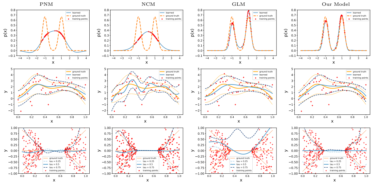
Figure 6.1: Details in Sec. 6.6 . ( top ) density estimation, ( center ) regression with Gaussian heteroscedastic errors. ( bottom ) multiple quantile regression. Shades of blue: estimated curves. Orange: ground truth. Models: ( left ) PNM, ( center-left ) NCM, ( center-right ), GLM, ( right ) Our model.
