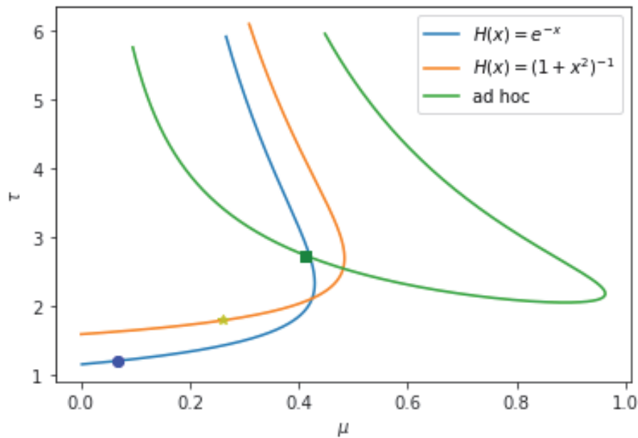
Figure 4.2: stability boundary for 3 functions (stable region on the right), represented in the coordinates (\mu, \tau) .
