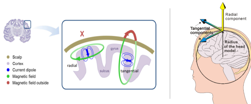
Figure 1.18: Left: Radial and tangential current dipoles and orientation of corresponding electric and magnetic field components. Taken from [Belaoucha 2017]. Right: Three orthogonal components of every current source. Taken from [Malmivuo et al. 1997].
