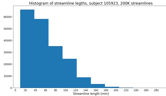
Figure 3.16: Histogram of streamline lengths, subject 105923.
