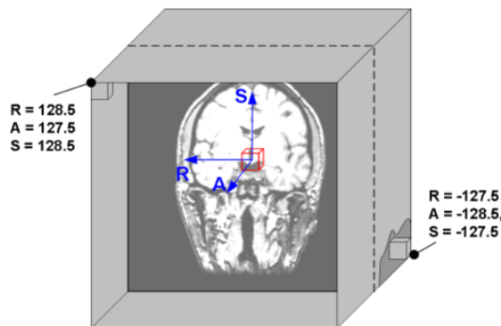
Figure 3.10: FreeSurfer MRI Surface RAS coordinates. Adapted from [Wideman 2003].
