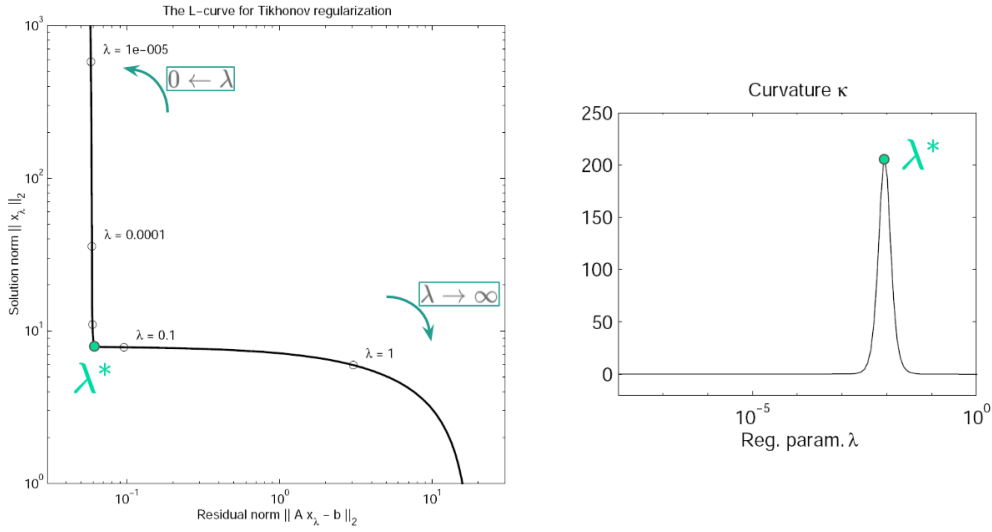
Figure 4.3: Left: A typical L-curve. The optimal \lambda^* (in green) chosen as the corner of the curve (point of maximal curvature). Right: Associated curvature function \kappa(\lambda) . Adapted from [Hansen 1999].
