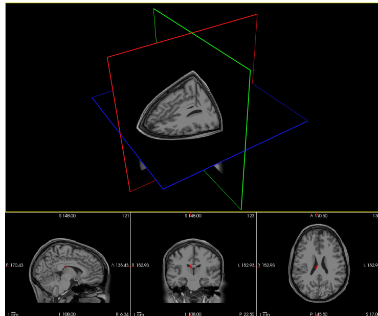
Figure 3.11: Up: intersection of anatomical planes. Down (from left to right): sagittal, coronal and axial view of slice with volume index (128, 128, 128), corresponding to the spatial position (0.0, 0.0, 0.0) mm in FreeSurfer surface RAS (which is (0.00, -17.50, 20.0) mm in NiBabel's scanner RAS). Recall that FreeSurfer surface mesh file contains metadata which indicates this shift between FreeSurfer RAS and NiBabel's scanner RAS.
