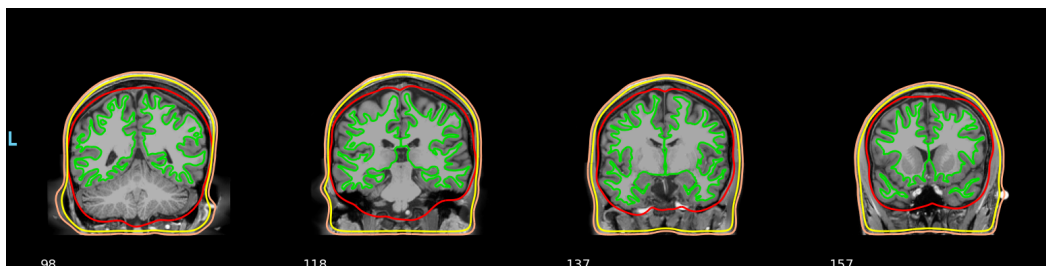
Figure 3.4: BEM contours overlaid on T1 image, representing the the scalp (orange), outer skull (yellow), intracranial space (red). White matter surface is shown in green.
