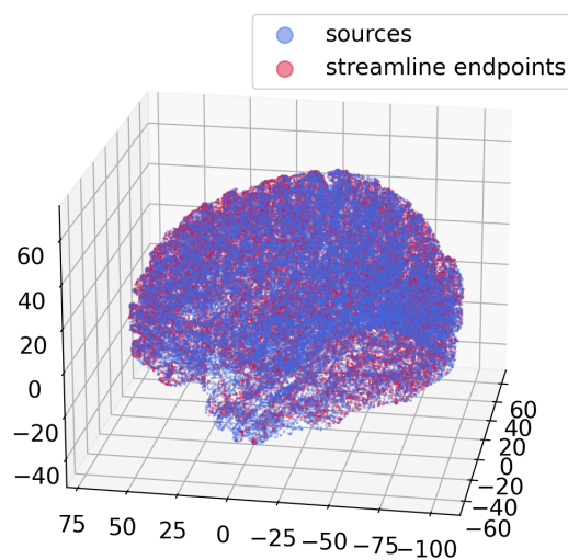
Figure 3.12: Alignment of source space dipoles with streamline endpoints (with axes in mm).
