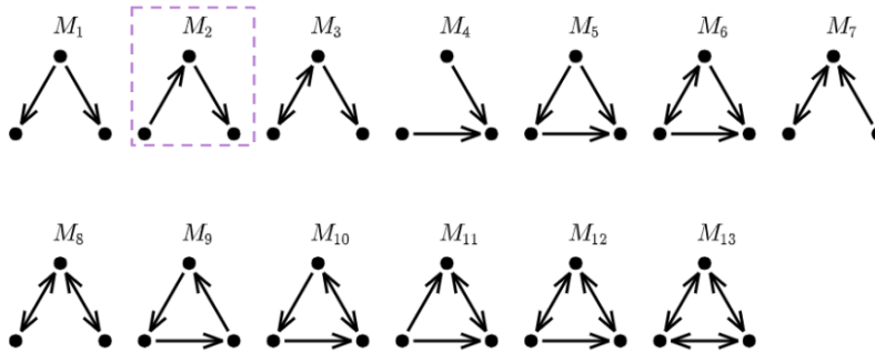
Figure 5.2: Network motifs: all 13 possible directed subgraphs of size 3, with all nodes connected. Adapted from [Xie et al. 2021]. Motif M_2 is highlighted as an example since it is also shown in Figure 5.1
