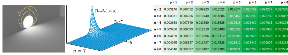
Figure 4.3: Illustration of Theorem 4.4.5: the radiant exitance operator T_b is not compact. Left: rendered scene with diffuse emitter S_n . Center: the radiant exitance computed on the receiver plane for n = 7 . Right: table contains the pairwise \mathcal{L}_2 distances between T_b B_n and T_b B_{n+p} .
