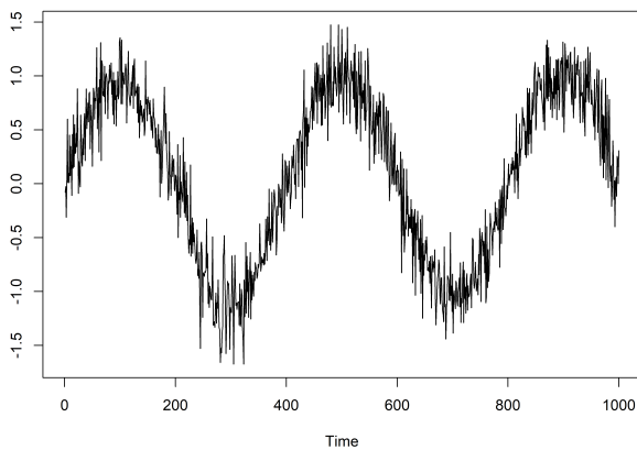
Figure 2.2: Influence of the bandwidth parameter h in nonparametric smoothing for functional data. Here the kernel used is the Gaussian kernel: K(x) = \frac{1}{\sqrt{2\pi}} \exp(-\frac{x^2}{2}) .
