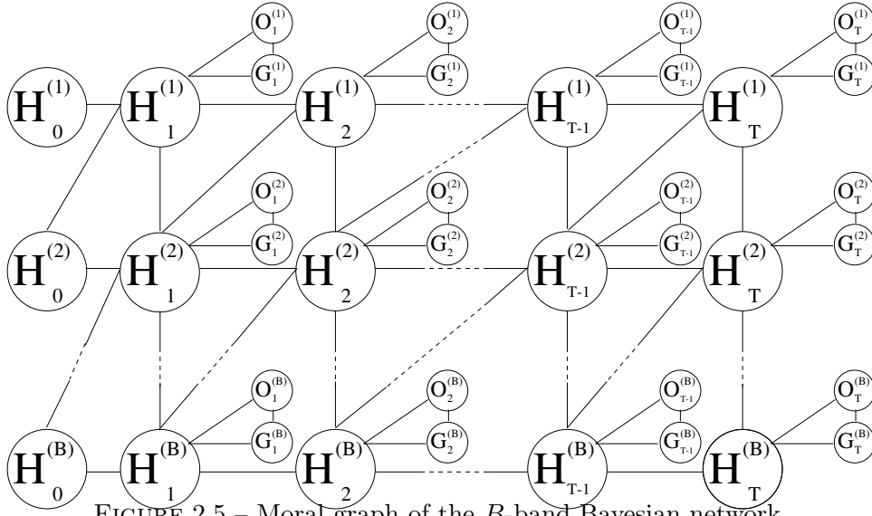
FIGURE 2.5 – Moral graph of the B -band Bayesian network.
