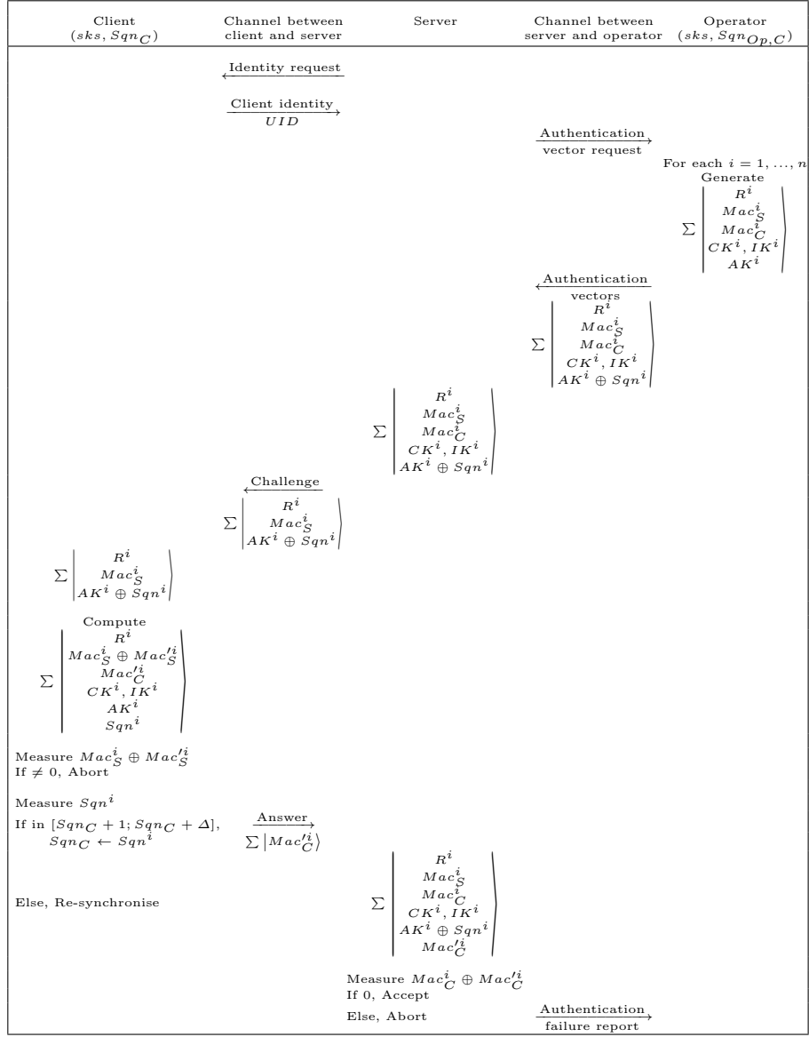
Fig. 2. Quantum version of the AKA protocol
