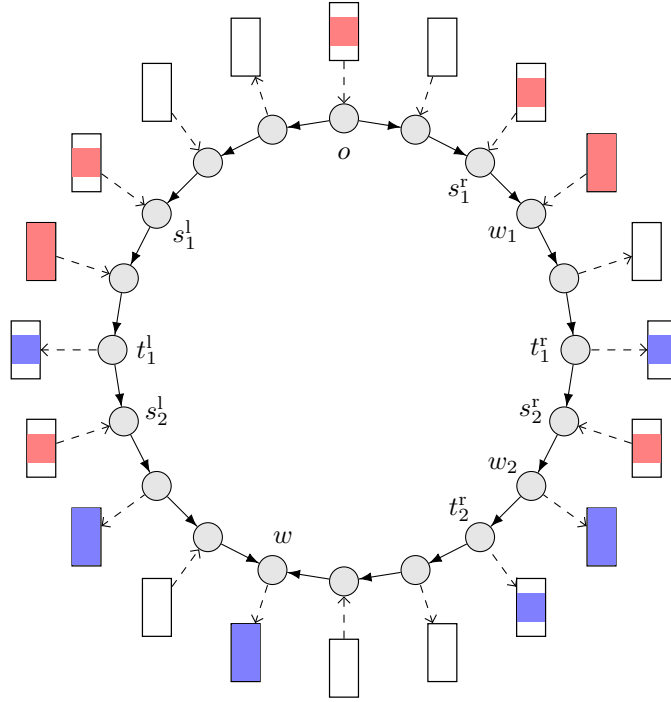
Figure 4.4: Configuration of s and t nodes with o \preceq_r w_1 \prec_r w_2 \preceq_r w (taken from [FP4]).
