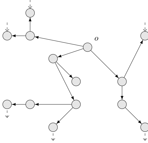
Figure 4.2: Example of a passive tree with all arcs directed away from the root o (adapted from [FP5]).
